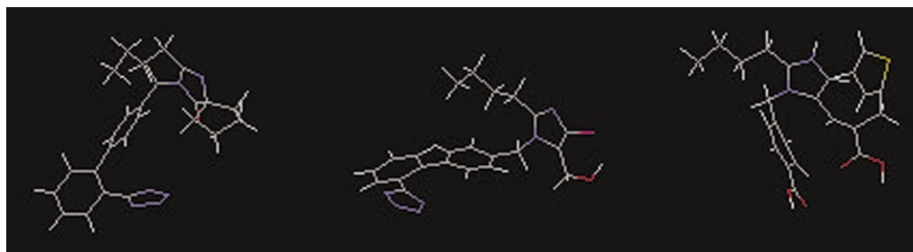
Figure 3. Low energy conformers of the three AT 1 antagonists losartan, eprosartan and irbesartan derived using a combination of NMR spectroscopy and computational analysis.
