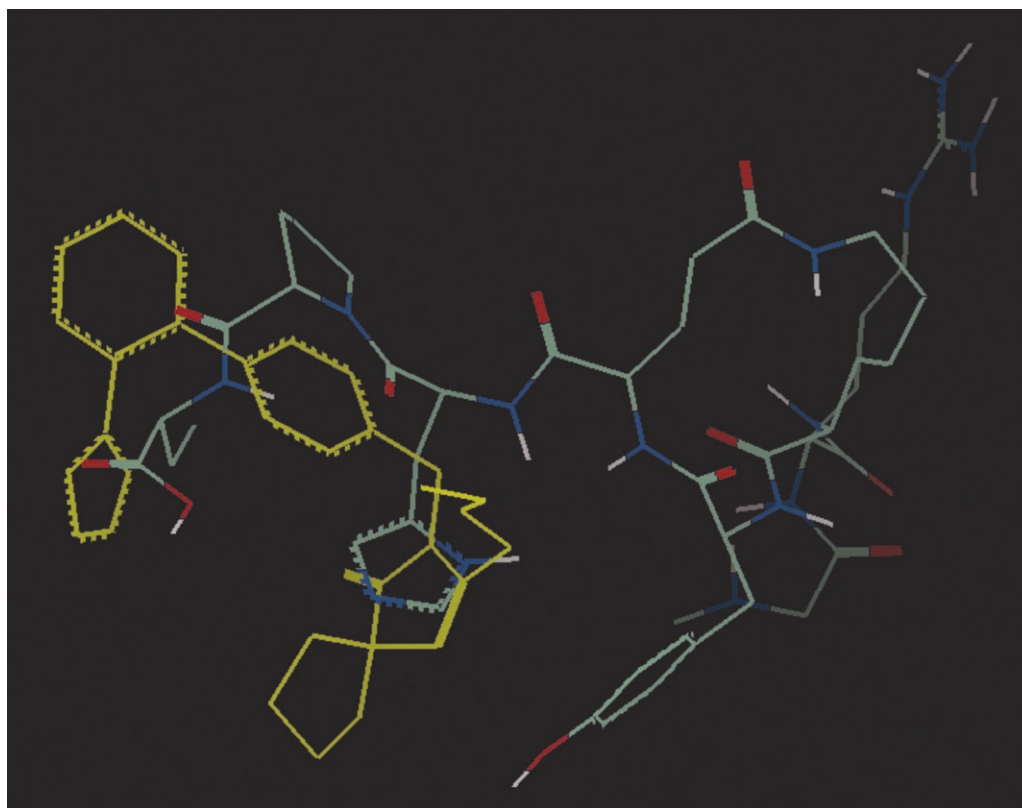
Figure 6. Superimposition of irbesartan with cyclic analogue 18.
