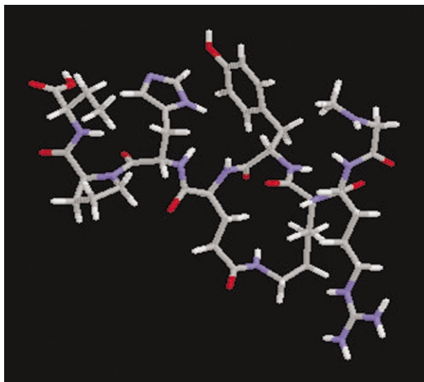
Figure 2. Low energy conformer of c(3,5)-[Sar 1 -Lys 3 -Glu 5 -Ile 8 ] ANG II.
