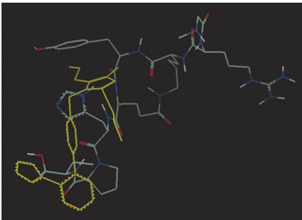
Figure 4. Superimposition of losartan with cyclic analogue 18 .
