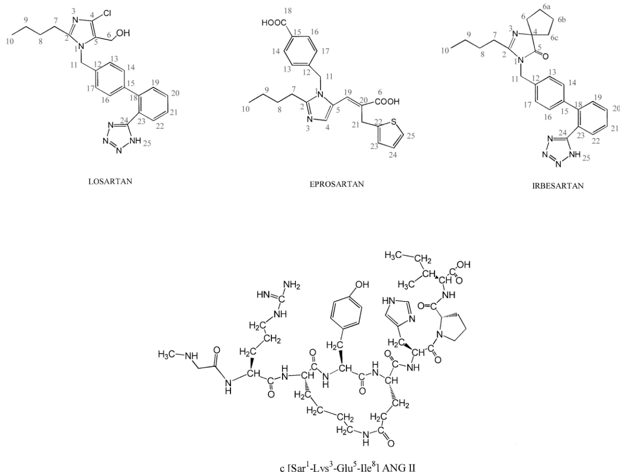
Figure 1. Chemical structures of cyclic compound 18 and AT 1 antagonists losartan, eprosartan and irbesartan.
