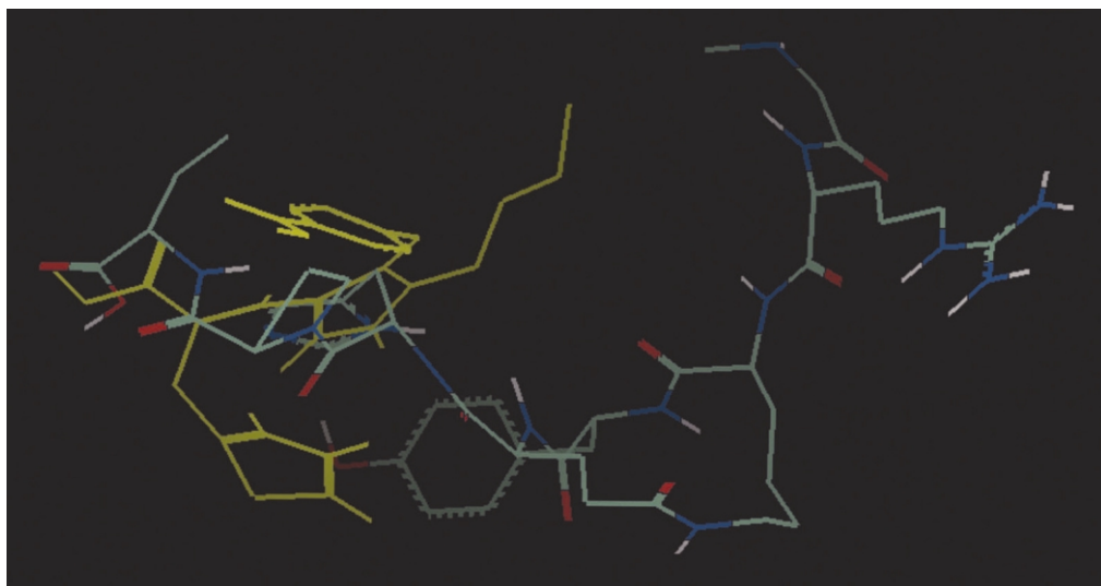
Figure 5. Superimposition of eprosartan with cyclic analogue 18.
