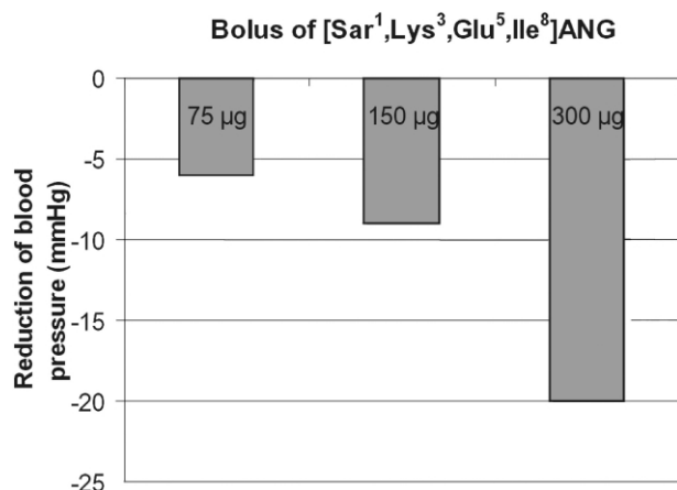
Figure 7. [Sar 1 -Lys 3 -Glu 5 -Ile 8 ] ANG II causes dose-related reduction of ANG II induced hypertension in anesthetized rabbits.
